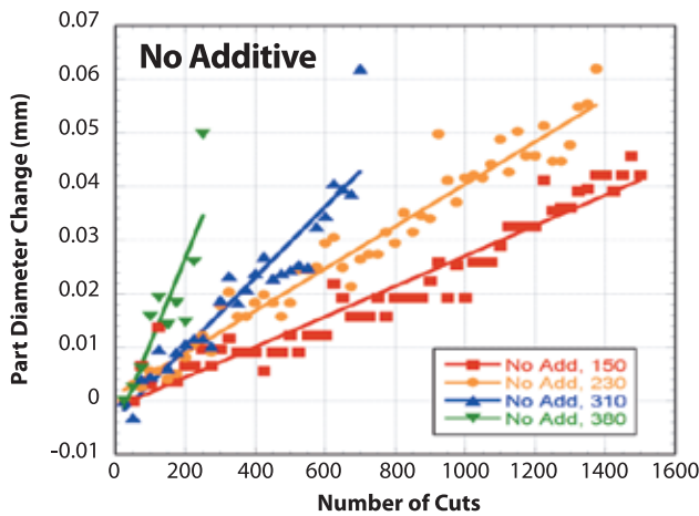
Improved Throughput in FC-0208
