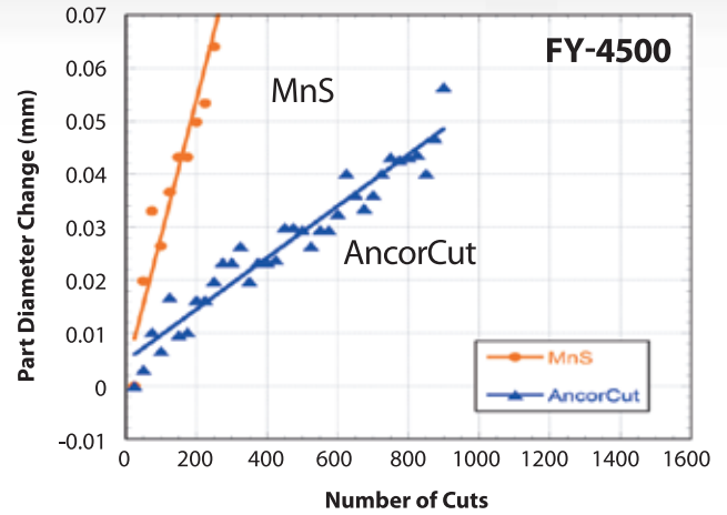
Reduced tool wear in FY-4500, FD-0405 and FLC2-4808
