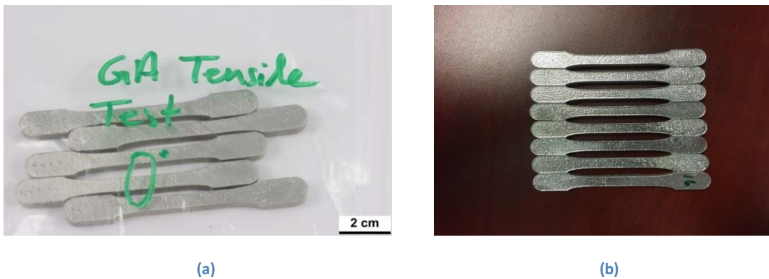
Figure 6(a) Picture of gas atomized tensile test specimens; (b) Picture of water atomized tensile test specimen
