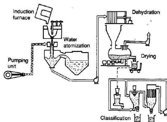
Figure 1. Schematic of the water atomization process [1]
