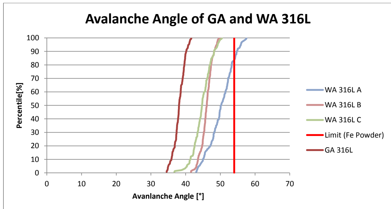
Figure 4. Graph depicting the behavior of the avalanche angle for each powder
