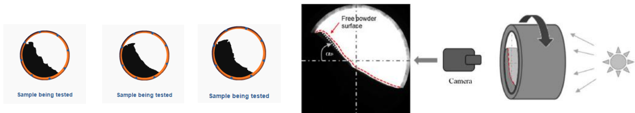
Figure 2. Schematic of the Powder Revolution Analyzer and how it functions [13]
