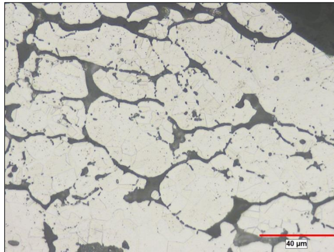
Figure 8. Picture of a 316L test piece microstructure highlighting the effects of nitrides on the microstructure
