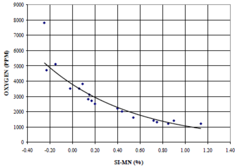
Figure 7. Relationship of silicon and manganese to oxygen content [1]
