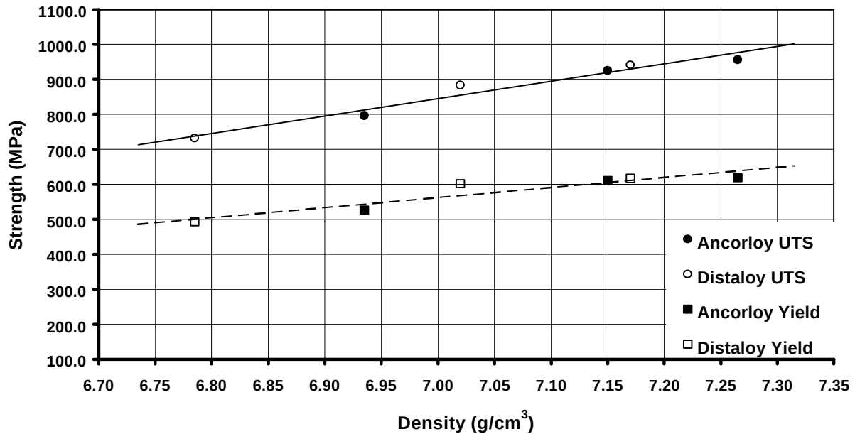
Figure 5 – Sintered and Tempered Yield and Ultimate Strengths of the HP Premixes
